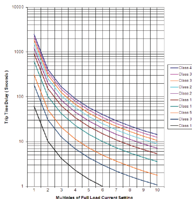
NewCode Thermal Trip Curve
