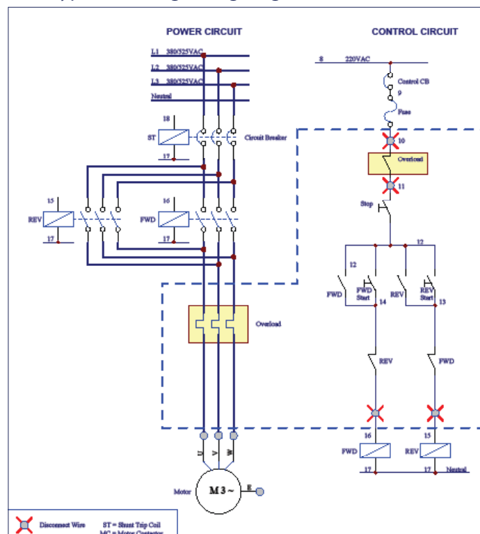
Typical existing wiring diagram of FWD/REV starter
